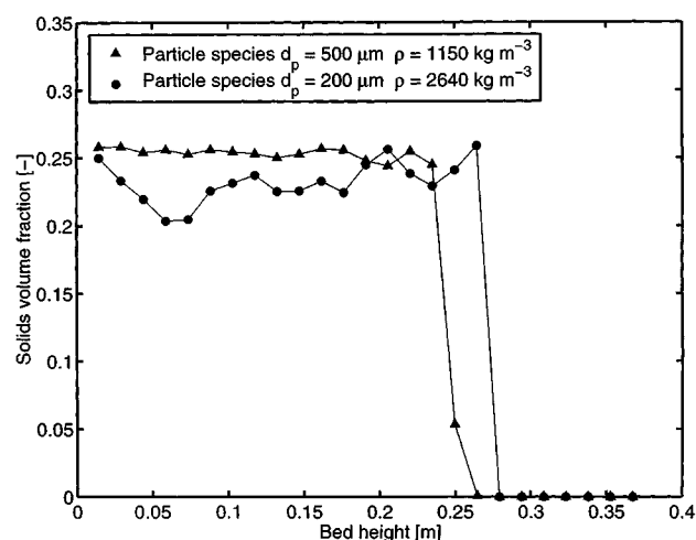
Figure 8. Strip- and 4 s time-averaged solids volume fraction of the bimodal mixture Case 2 fluidized bed at U = 1.85 m/s.
