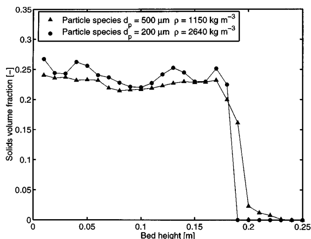
Figure 7. Strip- and 4 s time-averaged solids volume fraction of the bimodal mixture Case 2 fluidized bed at U = 1.08 m/s.
